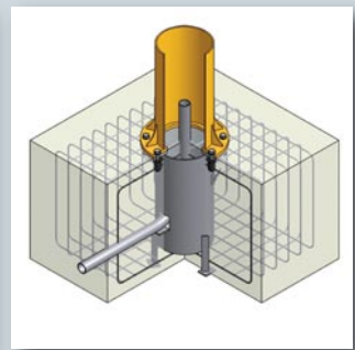
KompaktAnker CompactAnchor
